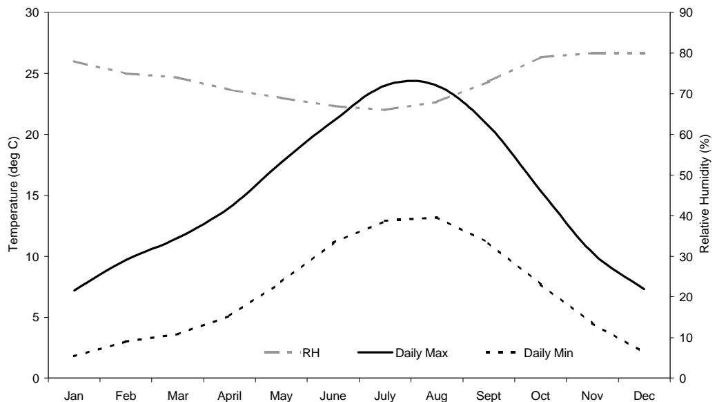
Figure 2.4 Temperature maximums and relative humidity for Seattle-Tacoma region
